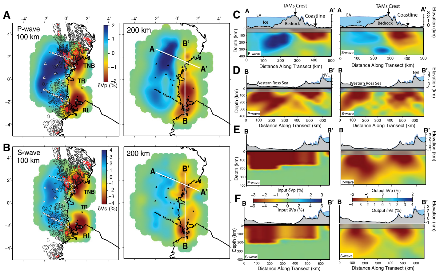
Figure 2. A, B: Map-view slices through our P-wave (A) and S-wave (B) models, highlighting velocity perturbations ( \delta V_p , \delta V_s ). Triangles denote stations (Fig. 1). On 100 km depth panels, black topographic contours represent 500, 1000, and 1500 m, and red contours represent 2000, 2500, and 3000 m from BEDMAP2 (Fretwell et al., 2013). Cross-section locations are shown on 200 km depth panels. TNB—Terra Nova Bay, TR—Terror Rift, RI—Ross Island. (C, D) Vertical cross sections along (C) profile A-A' and (D) profile B-B'. EA—East Antarctica; TAMs—Transantarctic Mountains; NVL—Northern Victoria Land. (E, F) The input and recovered models for the P-wave (E) and S-wave (F) synthetic tests.
