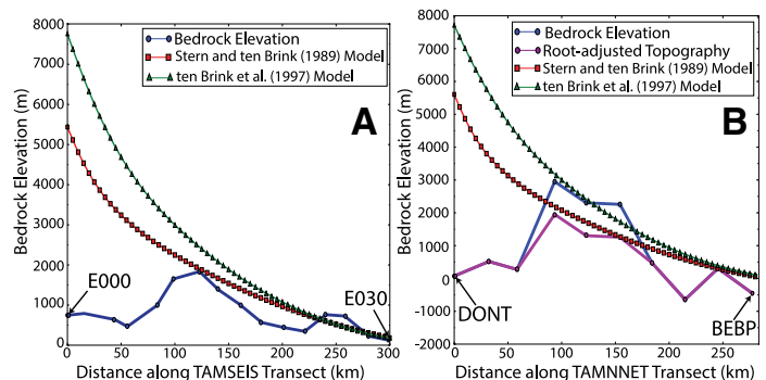
Figure 3. Bedrock topography from BEDMAP2 (blue lines; Fretwell et al., 2013) and modeled flexural profiles along the Transantarctic Mountains Seismic Experiment (TAMSEIS) (A) and the Transantarctic Mountains Northern Network (TAMNNET) (B) transects (Fig. 1). Red lines show 1989-equivalent model results, and green lines show 1997-equivalent model results. Purple line in B shows ~1 km adjusted bedrock topography. See text for details.
